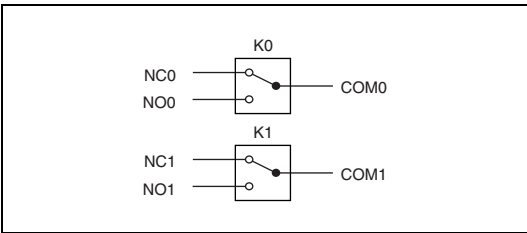
Figure 3. NI PXI-2599 Power-On State
