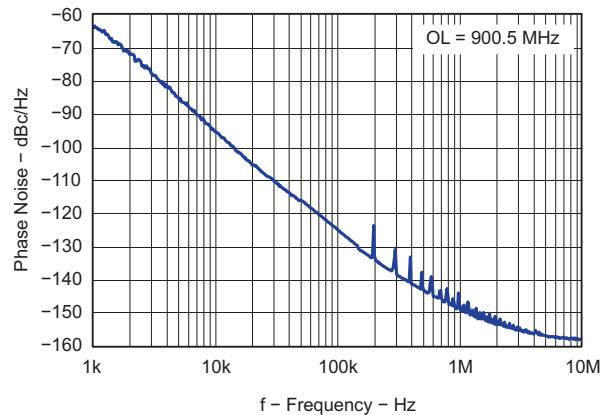
Figure 32. Open Loop VCO Phase Noise
