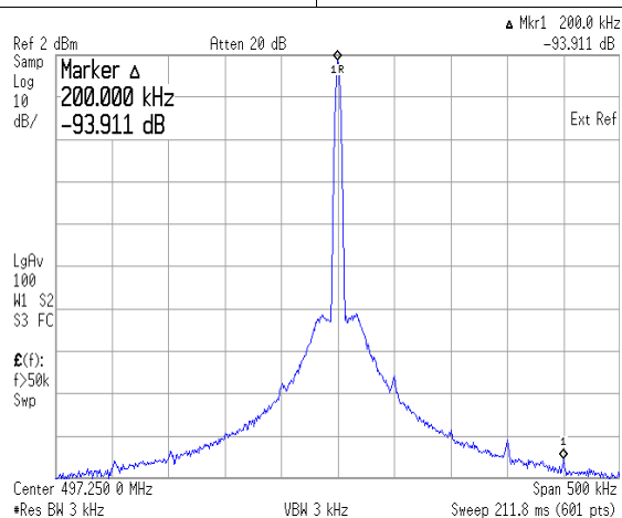
Figure 64. Divide-By-4 Output: PFD Frequency Spurs
