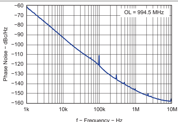
Figure 59. Open Loop VCO Phase Noise
