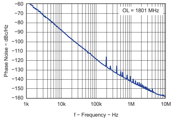
Figure 30. Open Loop VCO Phase Noise
