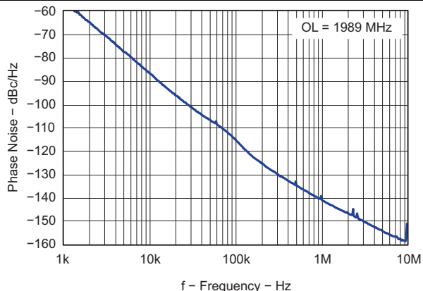
Figure 57. Open Loop VCO Phase Noise
