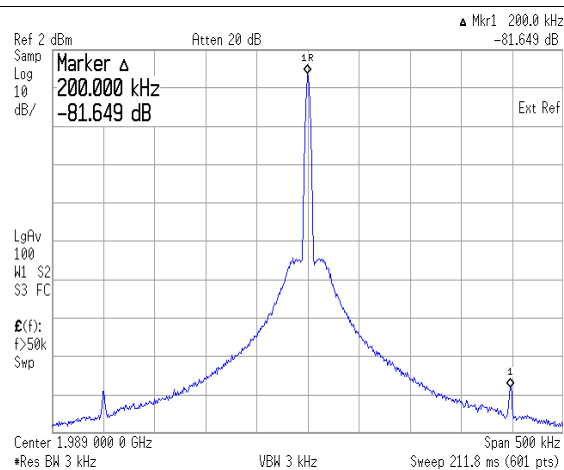
Figure 62. Direct Output: PFD Frequency Spurs
