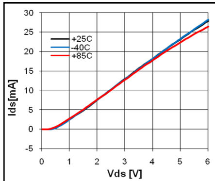
V-I Characteristics
