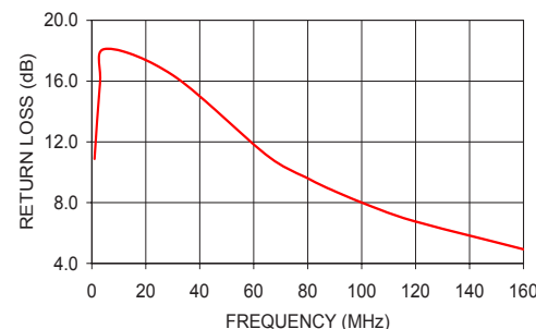
ADT16-1T INPUT RETURN LOSS
