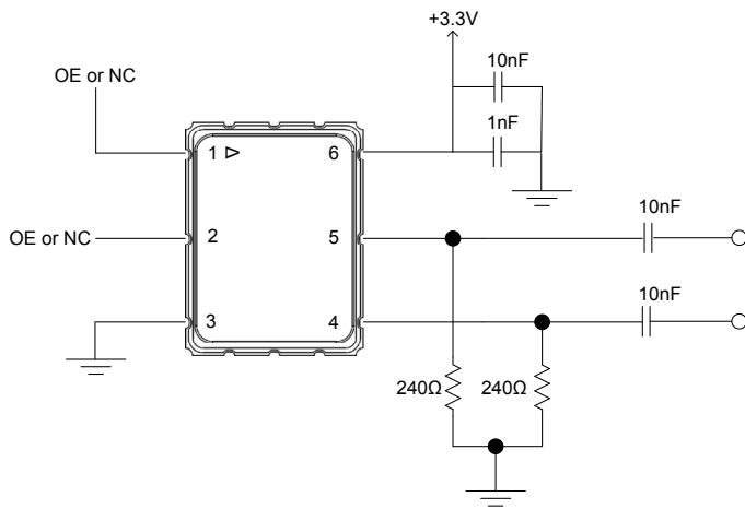
Figure 6 - Single Resistor Termination Scheme
