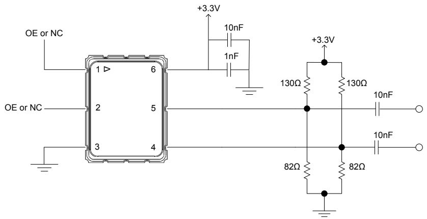
Figure 7 - Pull Up Pull Down Termination
