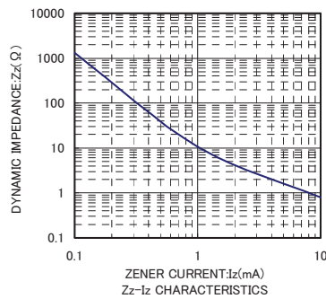
Zz-Iz CHARACTERISTICS
