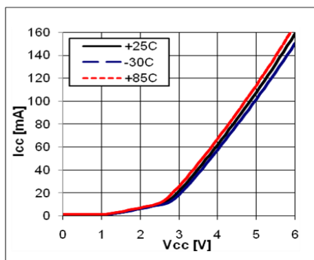
V-I Characteristics
