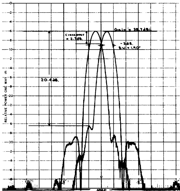
E-Plane — X-Band (48" Dia.)
