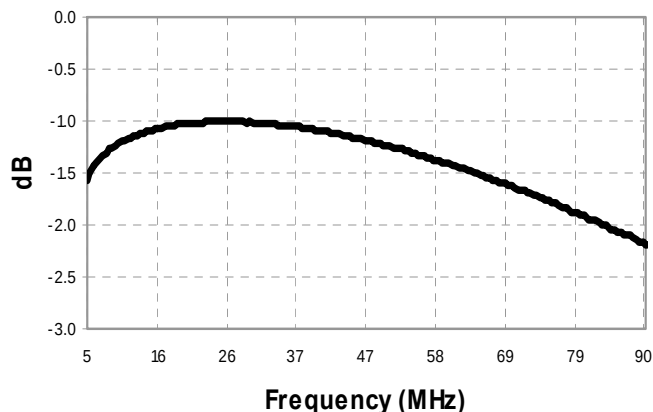
Amplitude Balance
