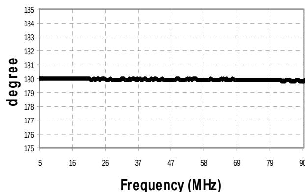
Phase Balance
