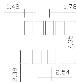
Footprint for PCB design
