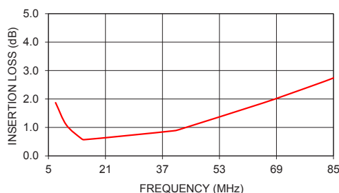
T16-1H+ INSERTION LOSS
