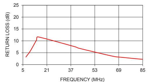
T16-1H+ RETURN LOSS
