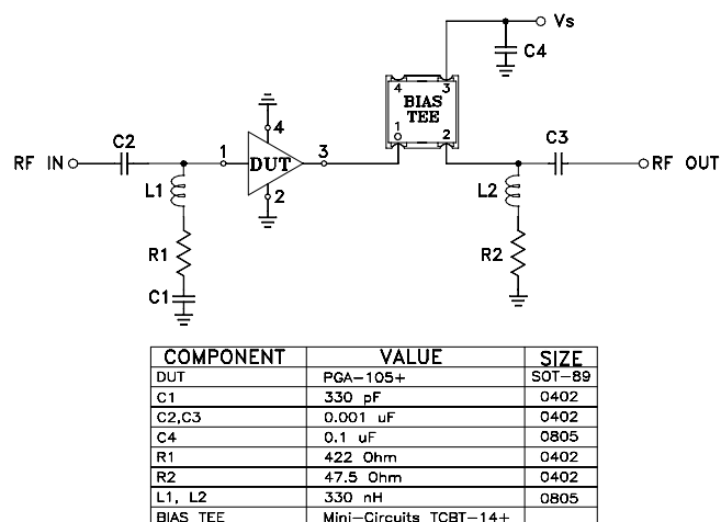
Fig 3. Evaluation board TB-733-105+ with unconditional stability (see applications note AN-60-063)
