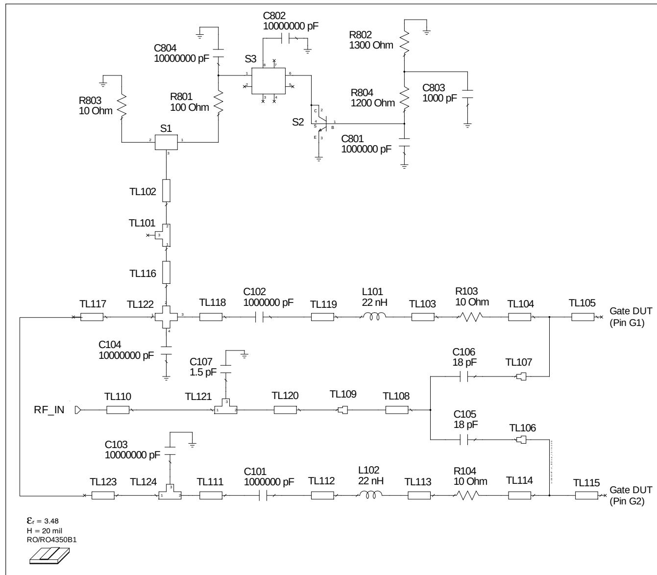
Reference circuit input schematic for f = 1990 MHz
