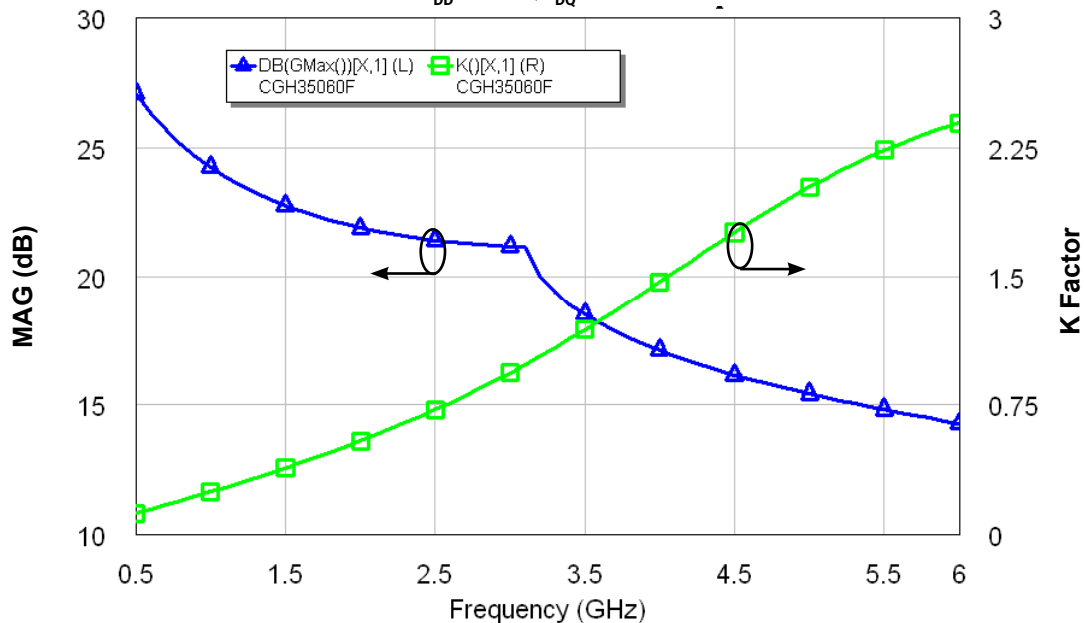
Simulated Maximum Available Gain and K Factor of the CGH35060F1 and CGH35060P1
