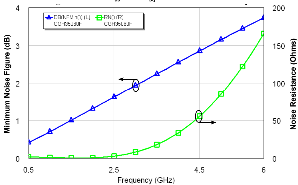
Simulated Minimum Noise Figure and Noise Resistance vs Frequency of the CGH35060
