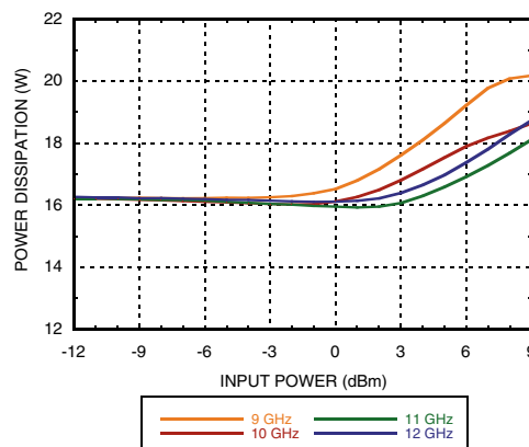
Power Dissipation
