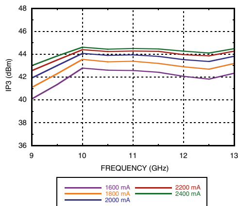
Output IP3 vs. Supply Current, Pout/tone = +20 dBm
