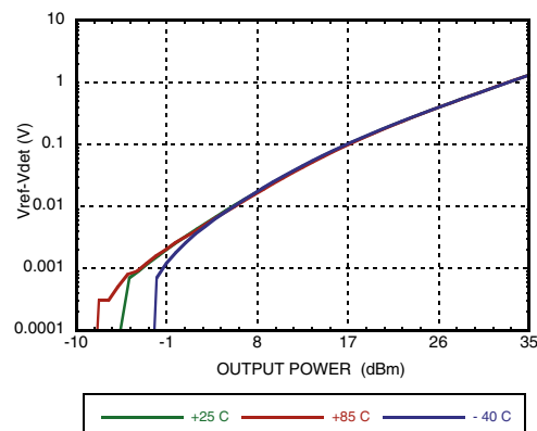
Detector Voltage vs. Temperature @ 9.5GHz
