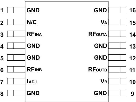
Figure 2: Pin Out
