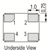
Underside View
