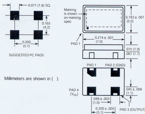
"T" Package
