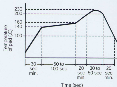
Recommended Reflow Soldering Profile
