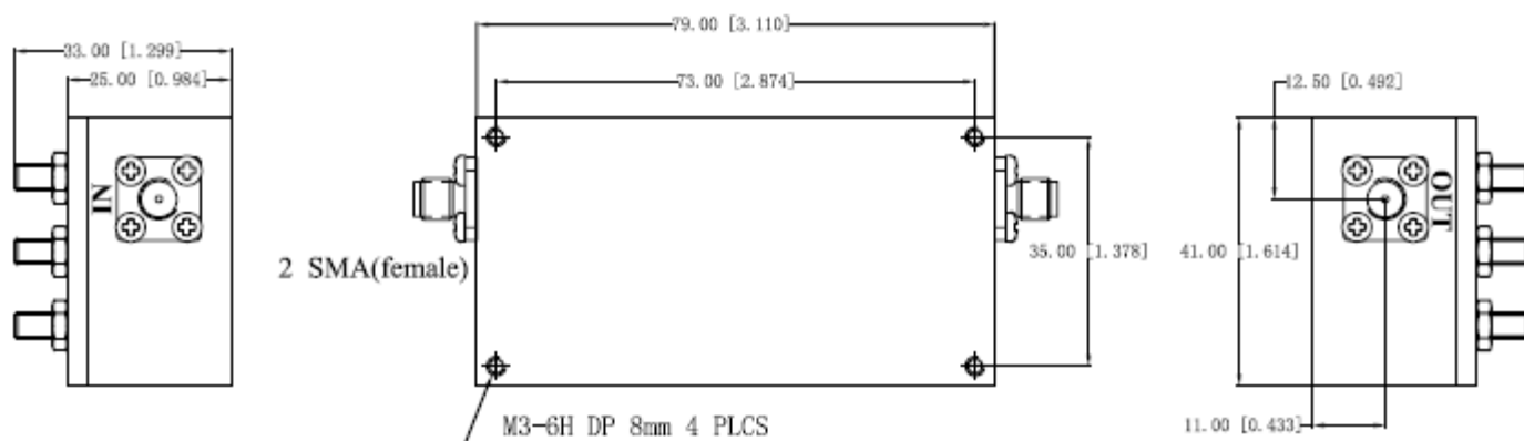
Outline Drawing
