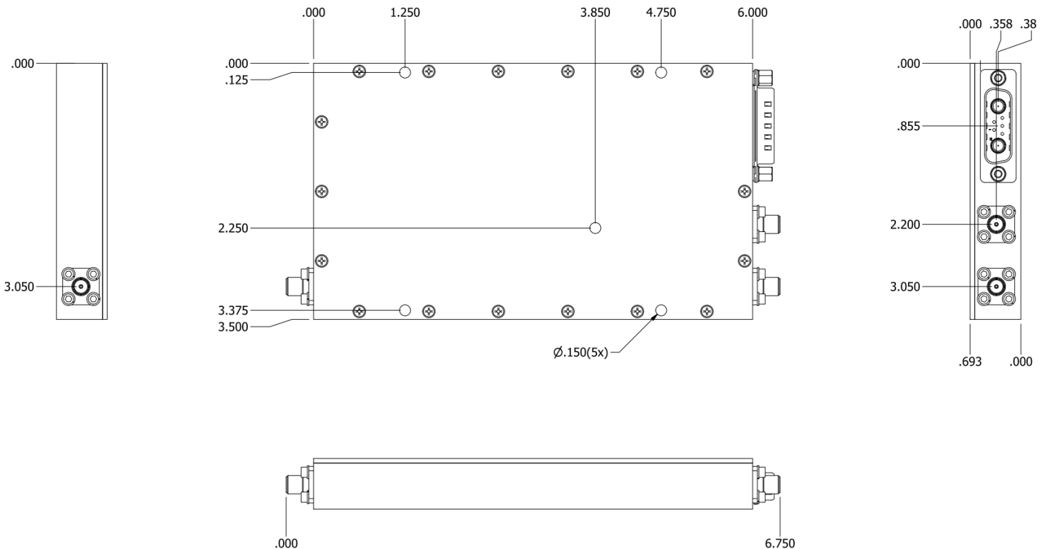
OUTLINE DRAWING
