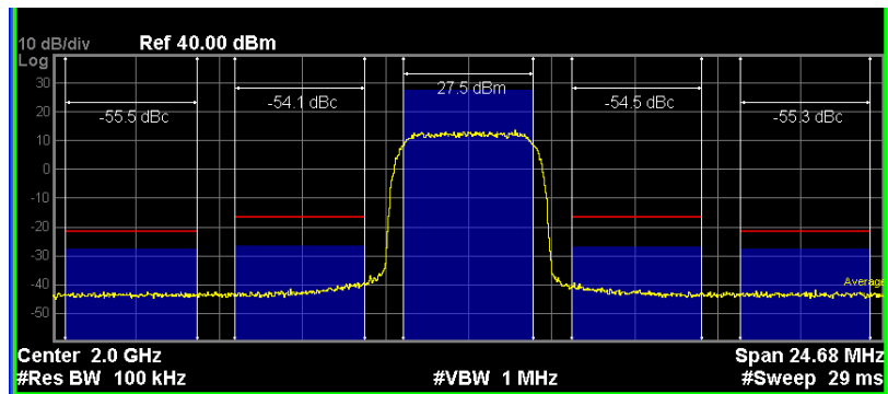
ACPR PLOT - 40.5 dBm W-CDMA
