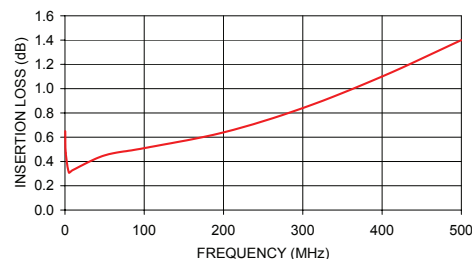
ADT4-5WT INSERTION LOSS
