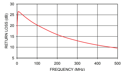
ADT4-5WT INPUT RETURN LOSS
