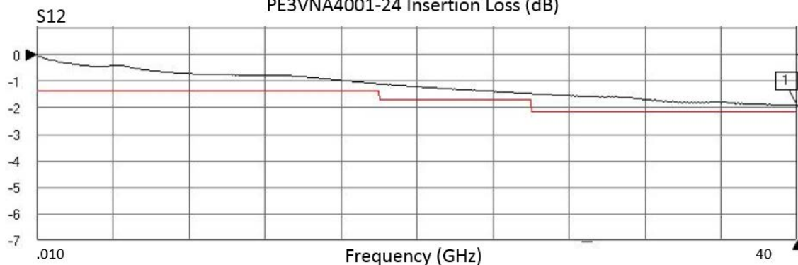
PE3VNA4001-24 Insertion Loss (dB)
