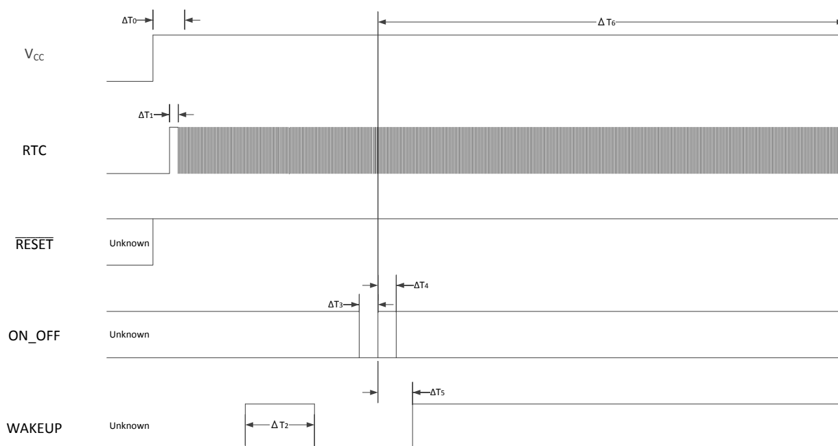
FIGURE 16 – START-UP TIMING
