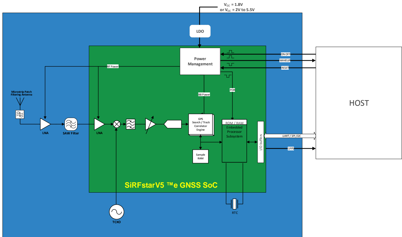
FIGURE 1 – ORG1510 ARCHITECTURE
