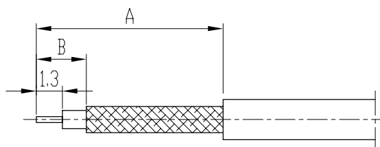
剥线尺寸 stripping dimensions
