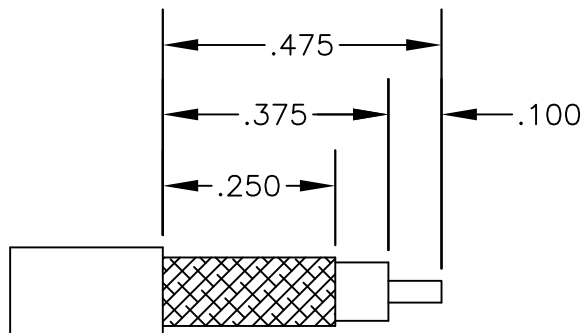
STRIPPING DIMENSIONS
