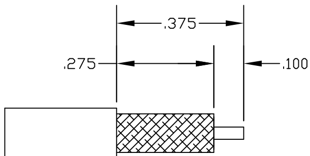
STRIPPING DIMENSIONS
