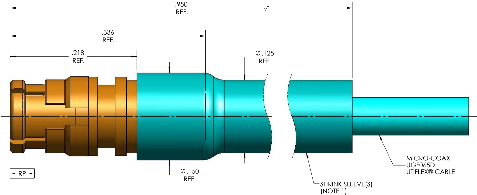
ISOMETRIC VIEW SCALE 4:1
