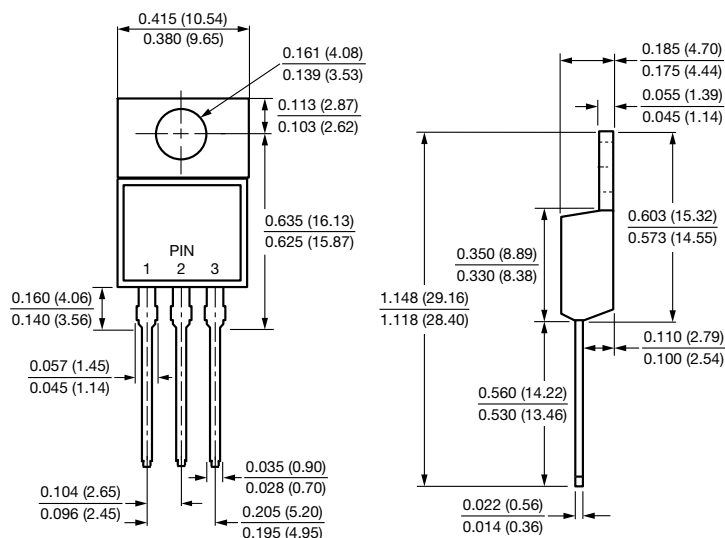
TO-220AB
