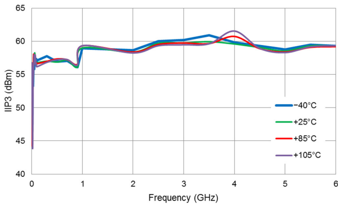
Input IP3 vs. Frequency
