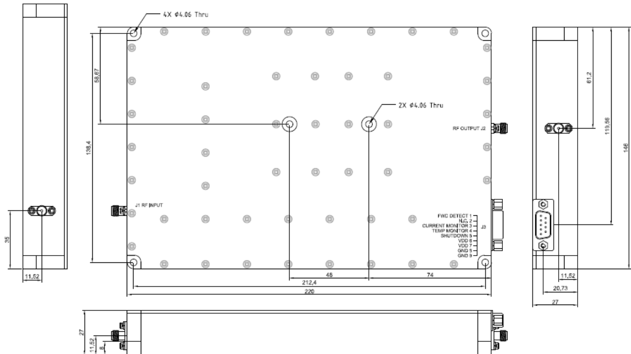
OUTLINE DRAWING - OPTION 01
