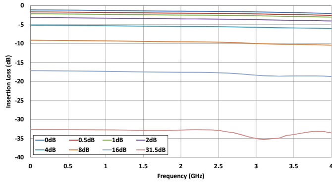
Figure 7. Insertion Loss vs Frequency @ Major Attenuation Steps
