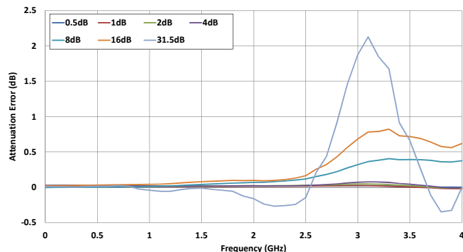
Figure 13. Attenuation Error vs Frequency @ Major Attenuation Steps
