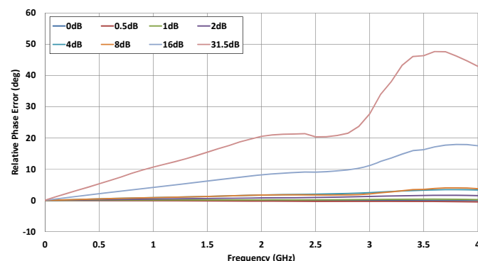
Figure 17. Relative Phase Error vs Frequency @ Major Attenuation Steps
