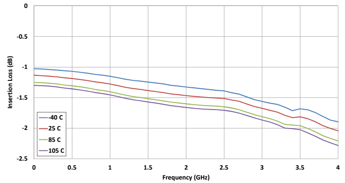
Figure 8. Insertion Loss vs Temperature
