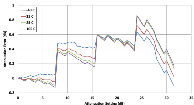
Figure 23. Attenuation Error @ 4 GHz vs Temperature
