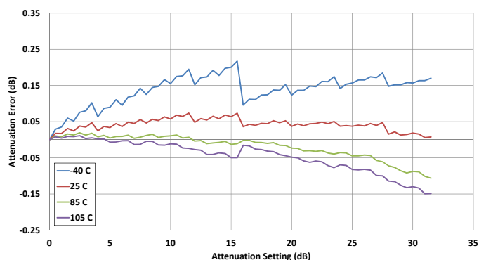
Figure 21. Attenuation Error @ 1 GHz vs Temperature
