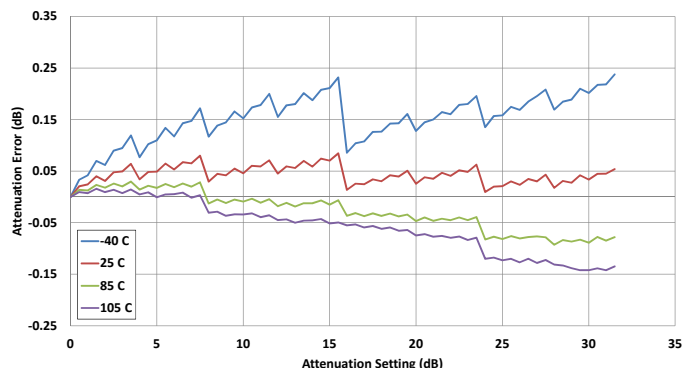
Figure 19. Attenuation Error @ 10 MHz vs Temperature
