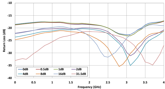
Figure 11. Output Return Loss vs Frequency @ Major Attenuation Steps
