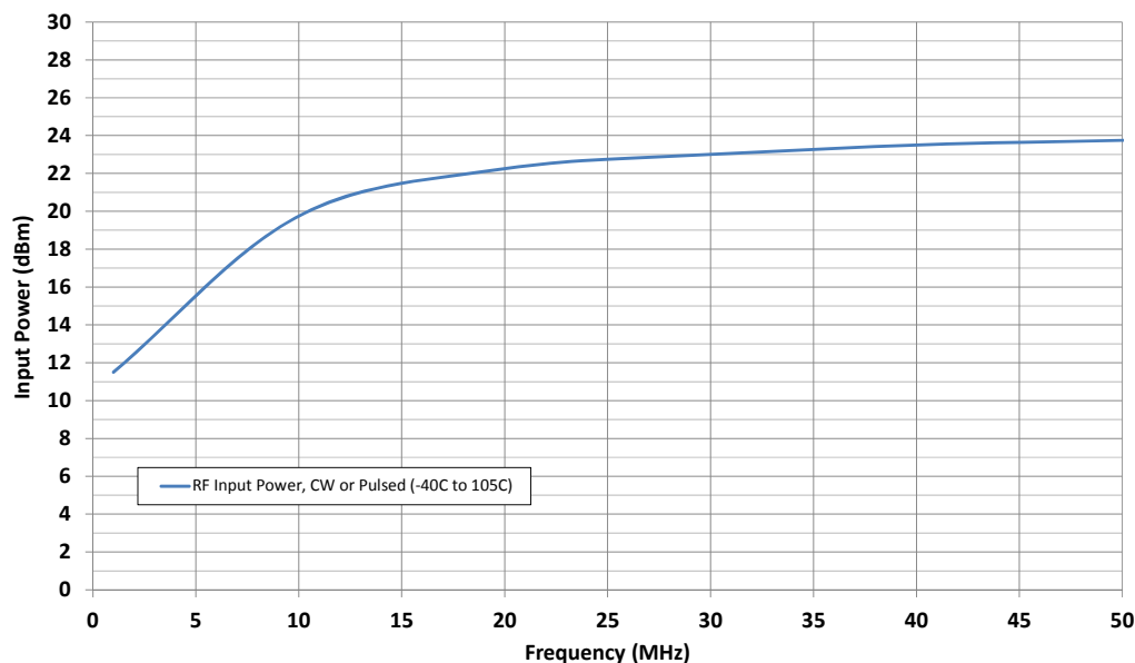
Figure 4. Power Derating Curve for 1 MHz – 50 MHz
