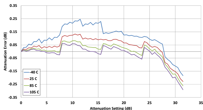
Figure 22. Attenuation Error @ 2.2 GHz vs Temperature
