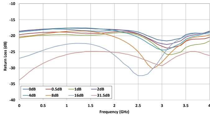
Figure 9. Input Return Loss vs Frequency @ Major Attenuation Steps
