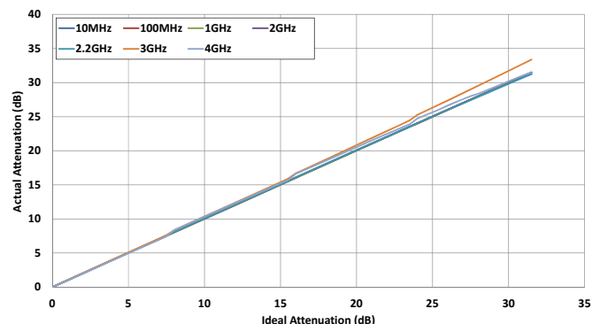
Figure 15. Actual Attenuation vs Ideal Attenuation
