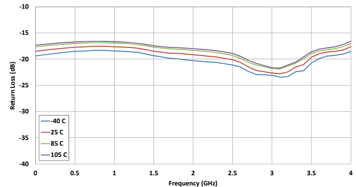
Figure 12. Output Return Loss vs Temperature
