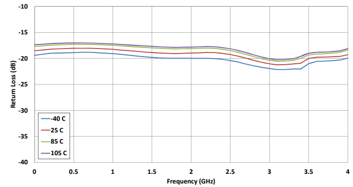
Figure 10. Input Return Loss vs Temperature
