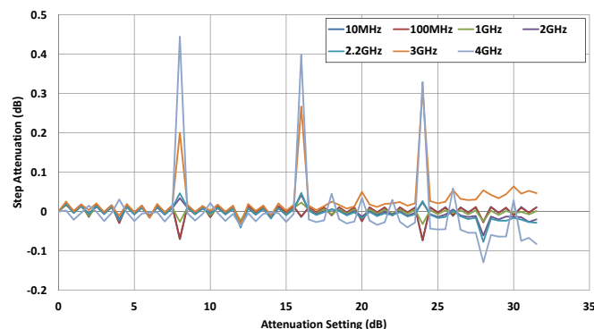
Figure 16. 0.5 dB Step Attenuation vs Attenuation Setting*
