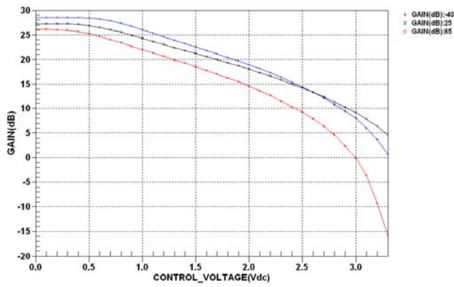
GAIN VS. CONTROL VOLTAGE VS. TEMPERATURE @ 1487.5 MHz
