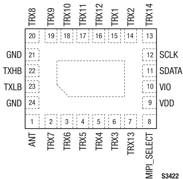
Figure 2. SKY13492-21 Pinout (Top View)
