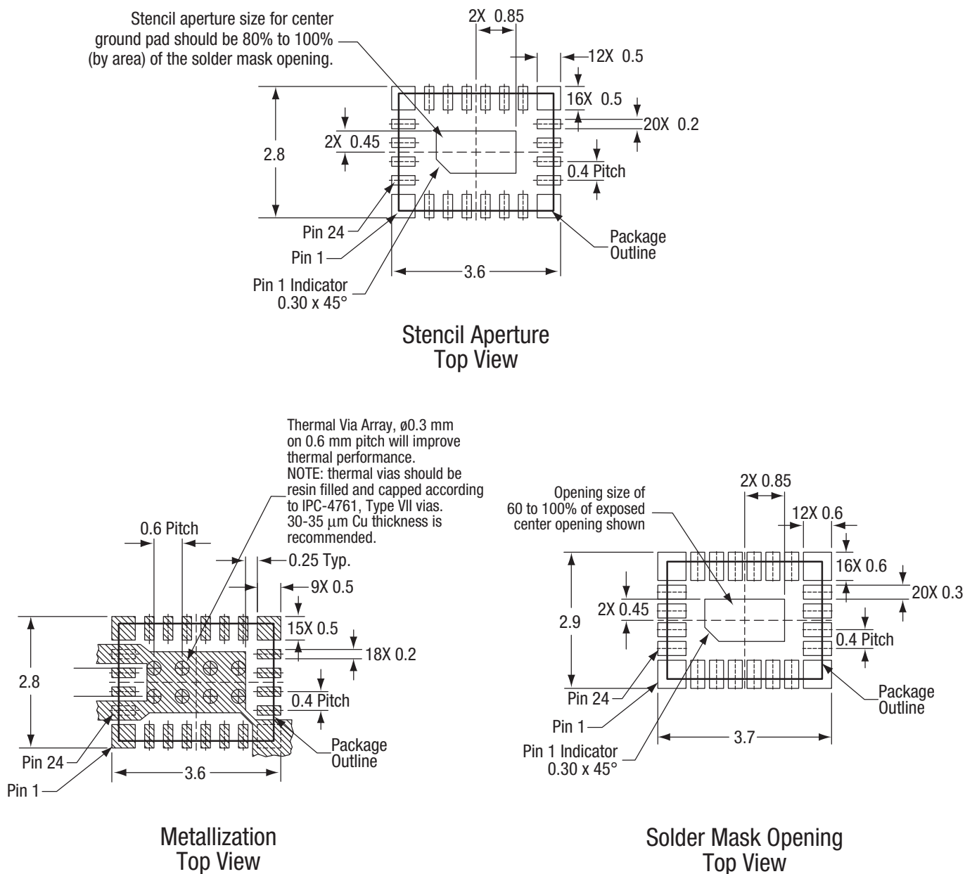
Figure 10. SKY13492-21 PCB Layout Footprint (Top View)
