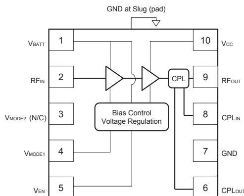
Figure 1: Block Diagram
