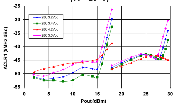
Figure 12: WCDMA ACLR1 (dBc) over Temperature ( T_c = 25\text{ }^{\circ}\text{C} )
