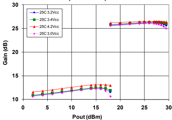
Figure 8: WCDMA Gain (dB) over Voltage ( T_c = 25\text{ }^{\circ}\text{C} )
