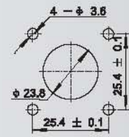
Mounting hole
