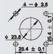
Mounting hole
