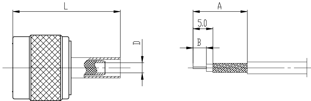
剥线尺寸 stripping dimensions
