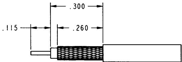
CABLE STRIPPING DIMENSIONS
