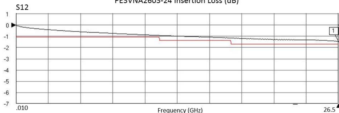
PE3VNA2603-24 Insertion Loss (dB)
