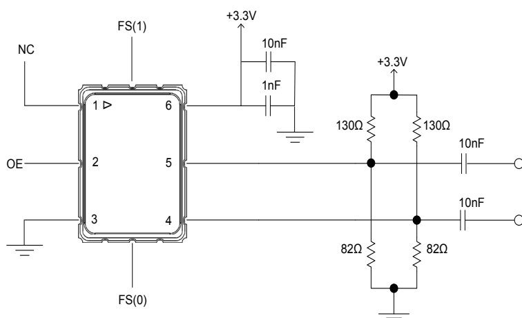
Figure 9 - LVDS to LVDS, External 100Ω and AC block ing caps
