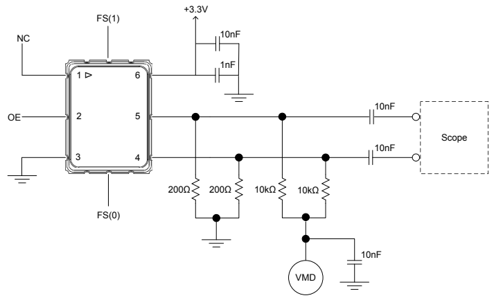
Figure 3 - LVPECL Production Test Circuit
