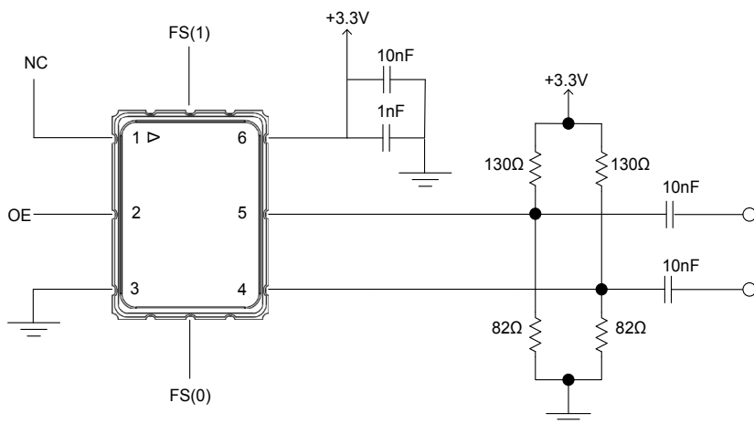
Figure 7 - Pull Up Pull Down Termination
