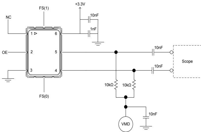
Figure 4 - LVDS Production Test Circuit
