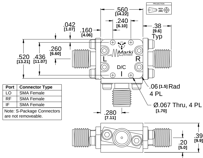
Outline Drawing – S package
