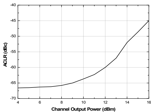
2140MHz ACLR Vs. Channel Output Power
