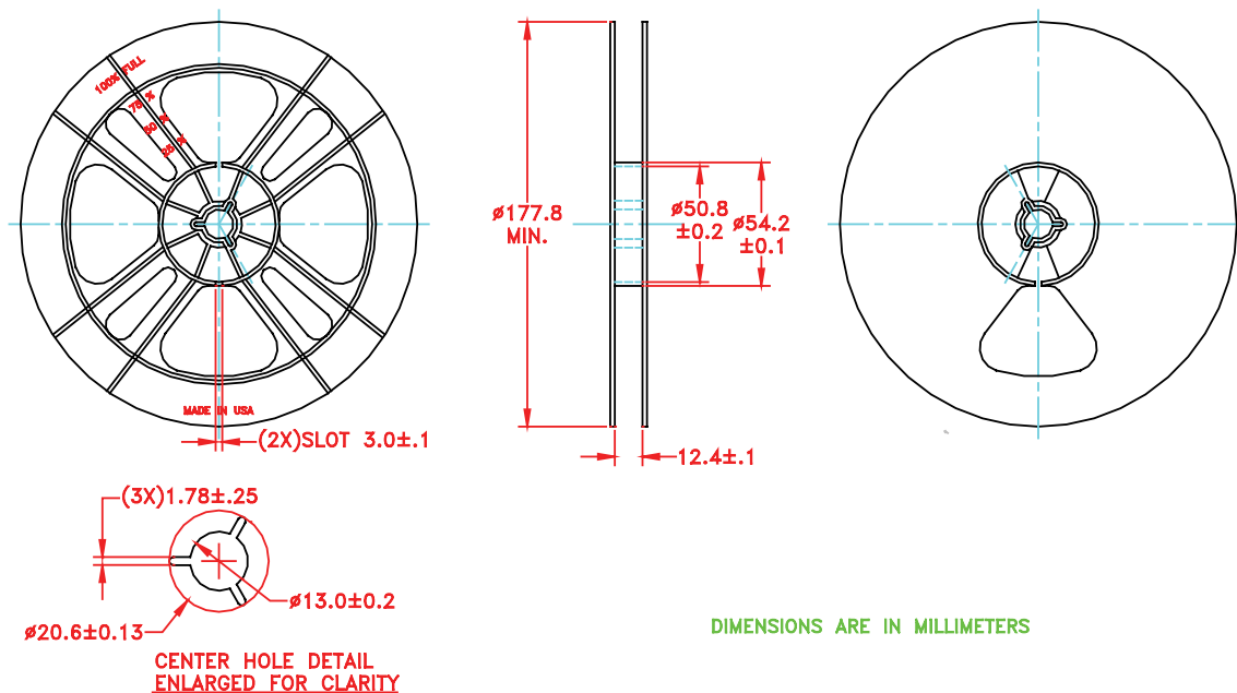
Figure 13: Carrier Tape
