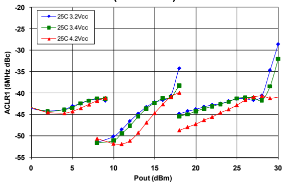
Figure 9: WCDMA ACLR1 (dBc) over Voltage ( T_c = 25 °C)
