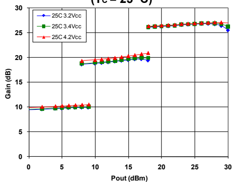
Figure 5: WCDMA Gain (dB) over Voltage ( T_c = 25 °C)
