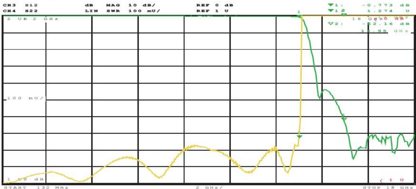
Frequency Response and VSWR
