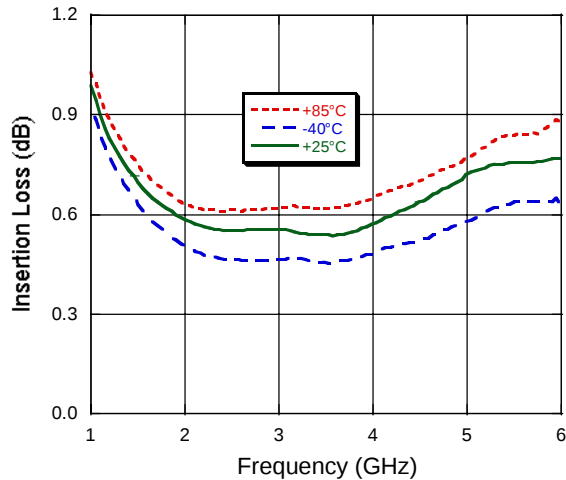
Insertion Loss
