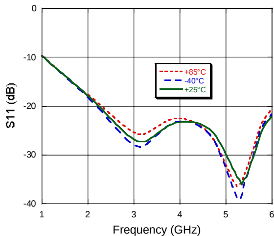
Return Loss
