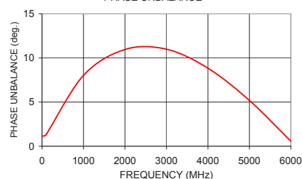
TCM1-63AX+ PHASE UNBALANCE
