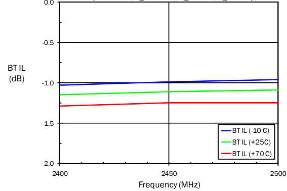
RF5611: BLUETOOTH MODE INSERTION LOSS versus FREQUENCY and TEMPERATURE (Vdd=3.3v, C_BT=2.8v, C_RX=0v, C_TX=0v)
