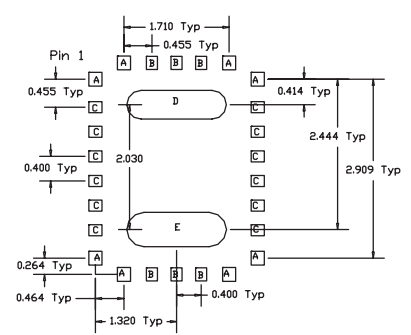
PCB STENCIL PATTERN
