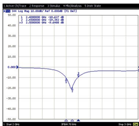
Antenna S11 on Test Board
