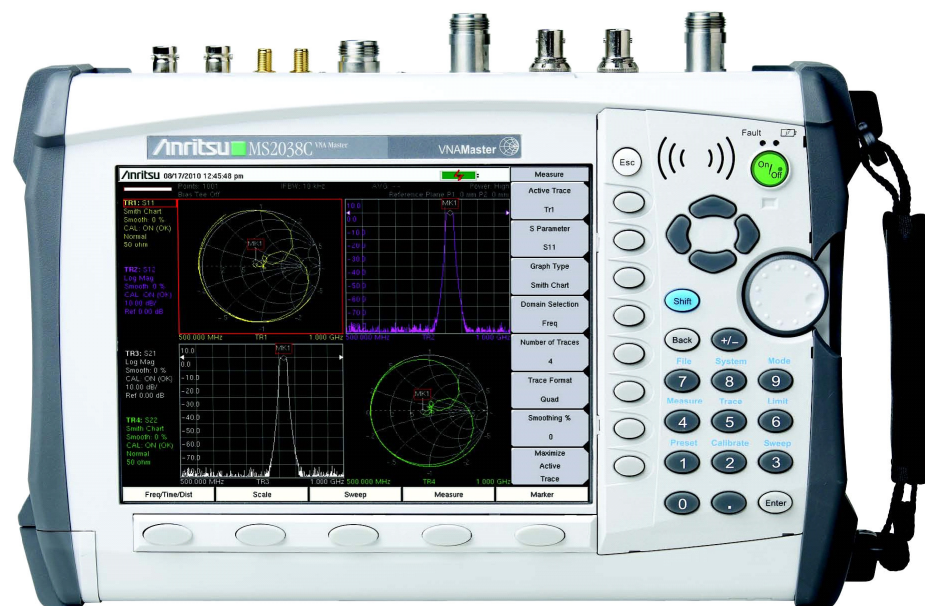
VNA Master TM MS202xC/MS203xC Vector Network Analyzer + Spectrum Analyzer
